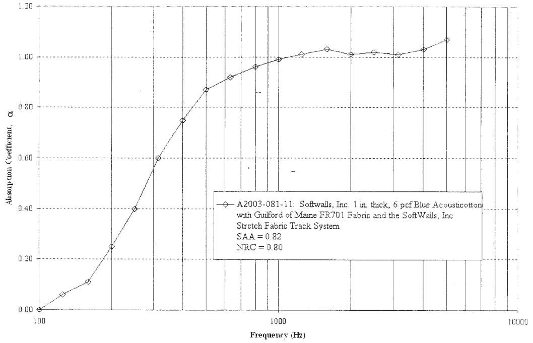
Graph 1. Sound Absorption Performance of SoftWalls, Inc. 1 in. thick, 6.0 pcf Blue Acousticotton with Guilford of Maine FR701 Fabric and the SoftWalls, Inc. Stretch Fabric Track System
